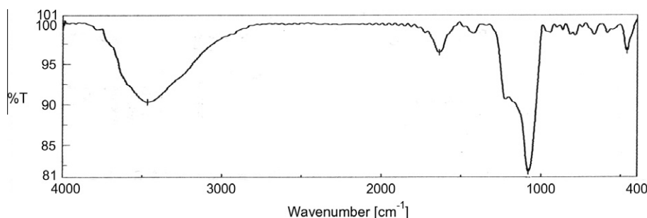
Figure 6 FTIR spectra of Cu-Al-MCM-41.
