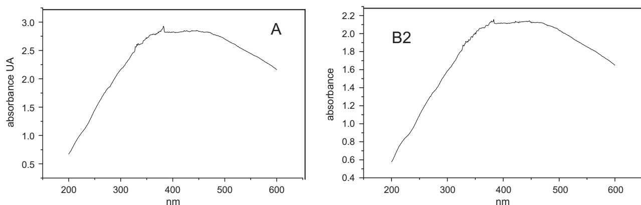
Figure 5 DR-UV-vis spectra of: (A2) calcined Cu-Si-MCM-41 and (B2) calcined Cu-Al-MCM-41.
