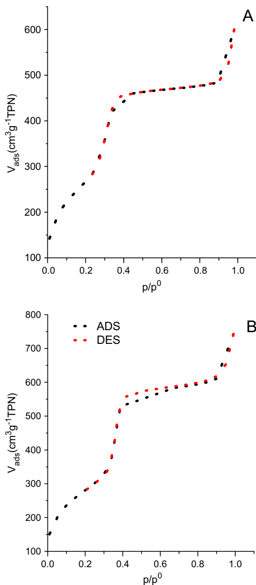
Figure 2 \text{N}_2 physisorption isotherms of (A) Si-MCM-41 and (B) Al-MCM-41.
