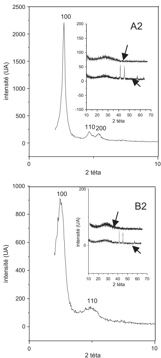
Figure 3 X-ray powder diffraction pattern of (A2) Cu-Si-MCM-41 and (B2) Cu-Al-MCM-41.
