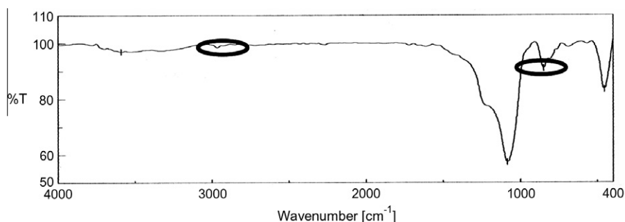
Figure 7 FTIR spectra of TMCS-Cu-Al-MCM-41.
