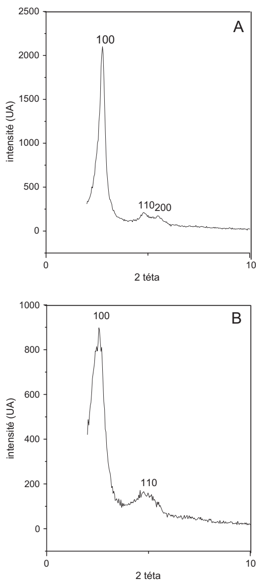
Figure 1 X-ray powder diffraction pattern of (A) Si-MCM-41 and (B) Al-MCM-41.
