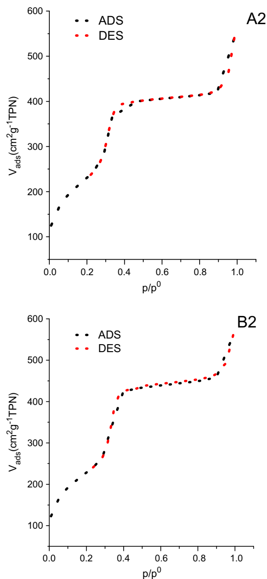
Figure 4 N 2 physisorption isotherms of (A) Cu-Si-MCM-41 and (B) Cu-Al-MCM-41.
